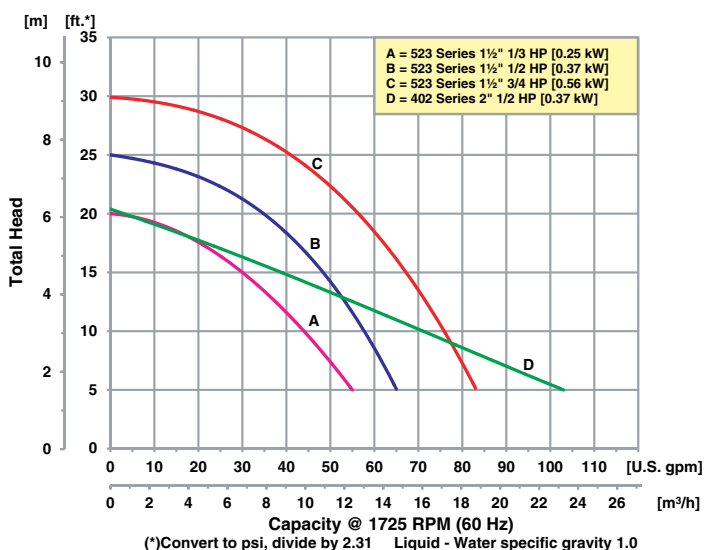
Performance of Industrial/Commercial Sump Pumps
