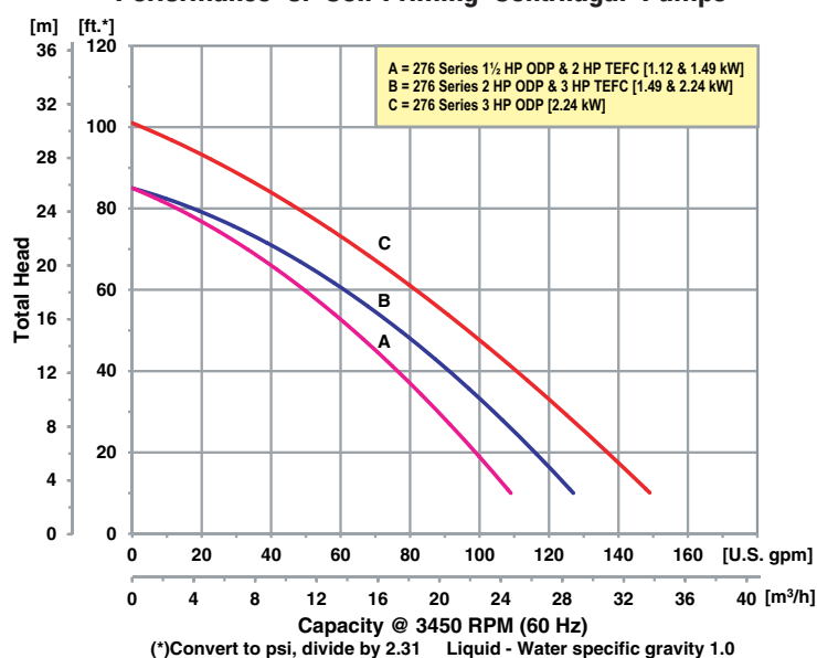
Performance of Self-Priming Centrifugal Pumps
