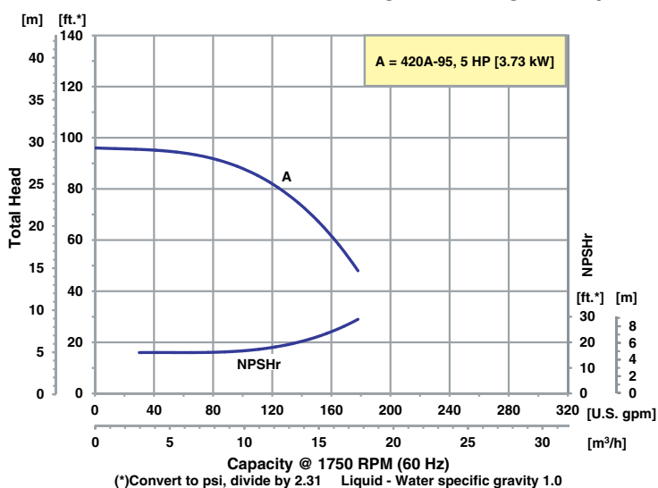
Performance of 2" x 1-1/2" Straight Centrifugal Pump
