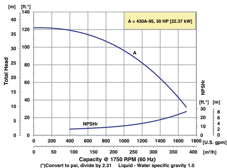
Performance of 6" x 4" Straight Centrifugal Pump
